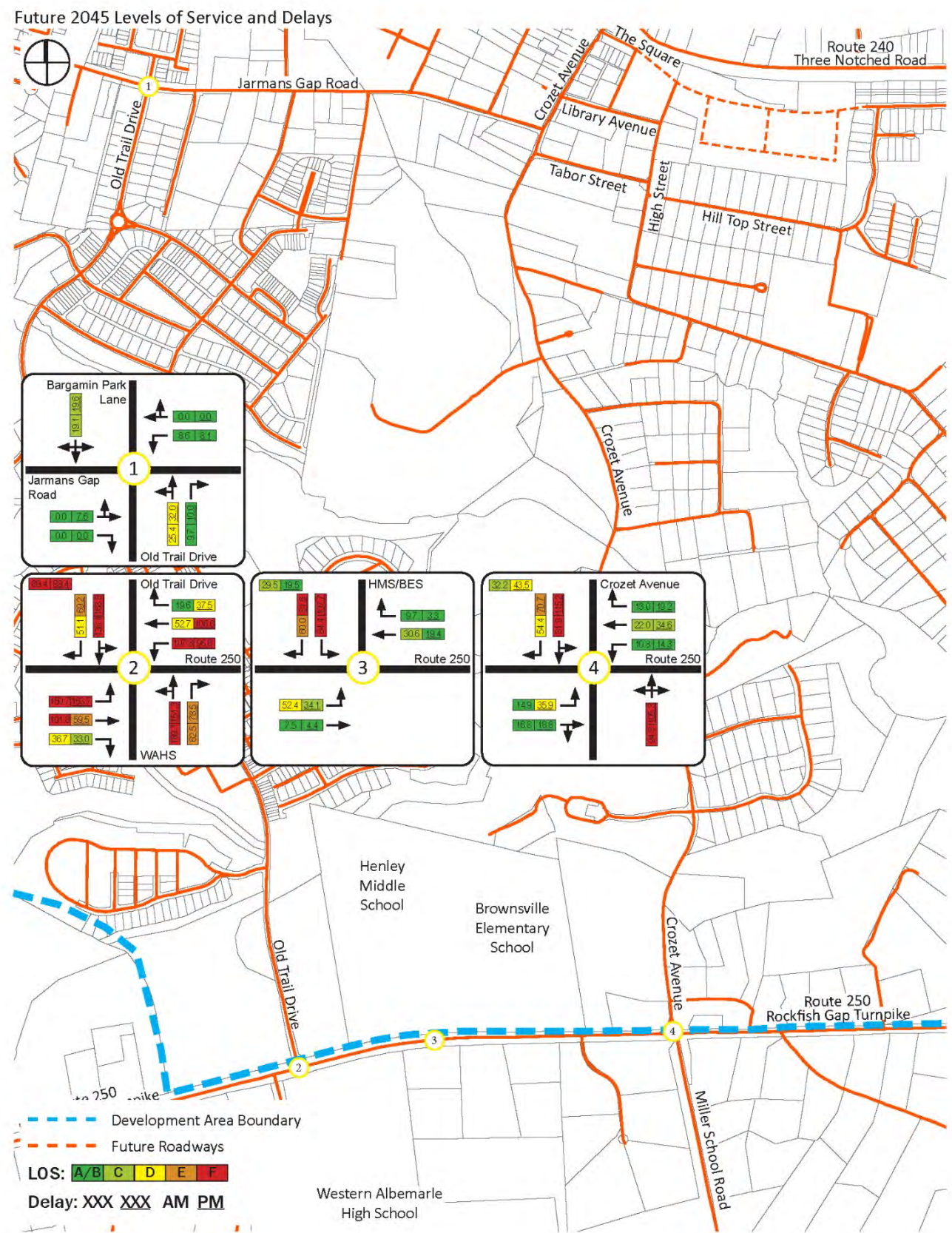
Figure 21 – 2045 Levels of Service and Delays Intersections 1-4
