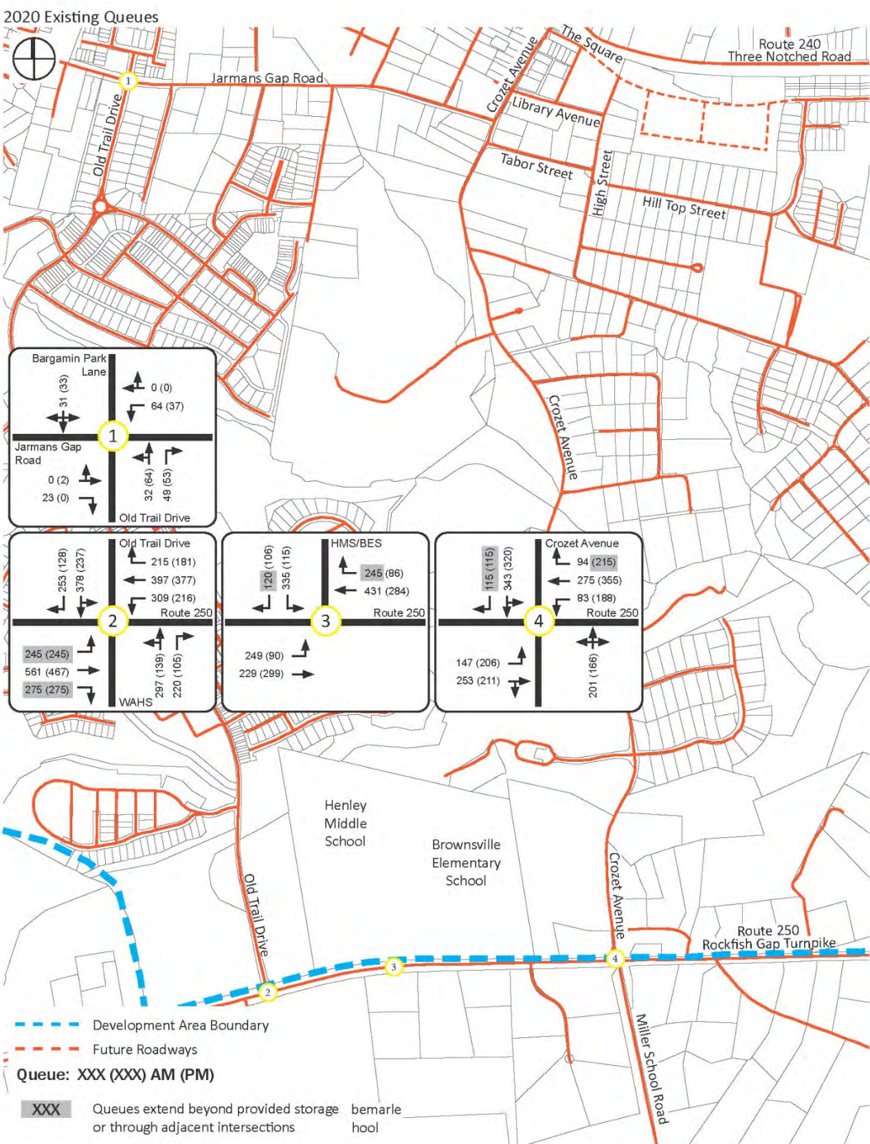
Figure 10 – 2020 Existing Queues Intersections 1-4
