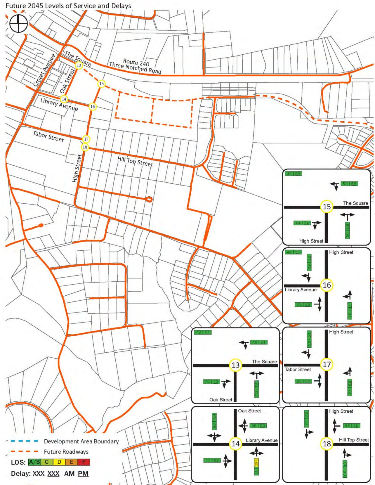
Figure 27 – 2045 Levels of Service and Delays Intersections 13-18
