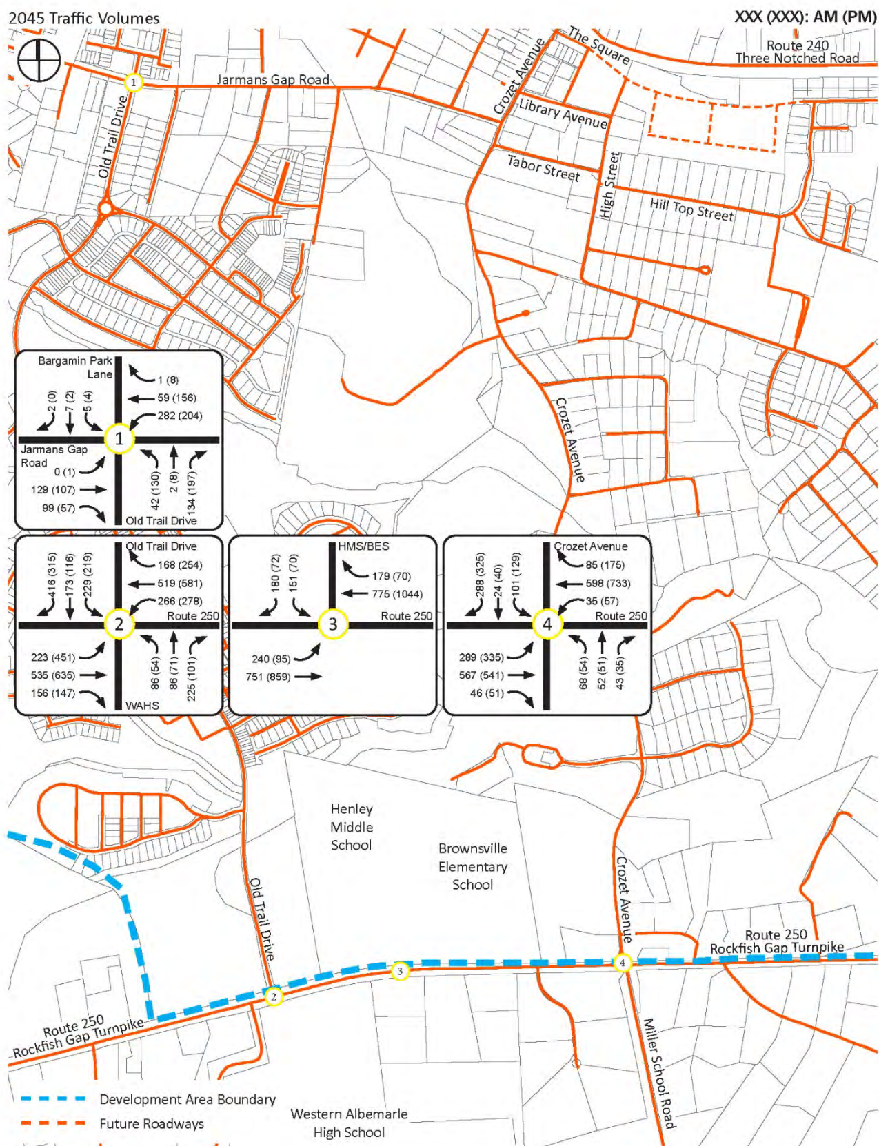
Figure 17 – 2045 Peak Hour Traffic Volumes Intersections 1-4
