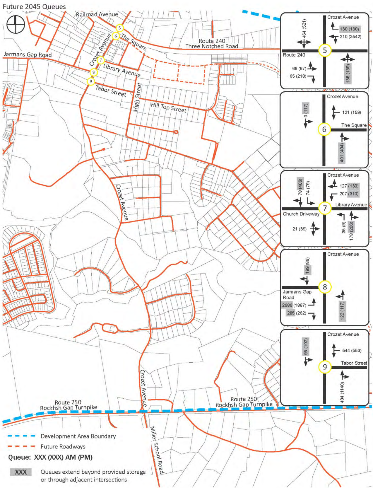
Figure 24 – 2045 Queues Intersections 5-9
