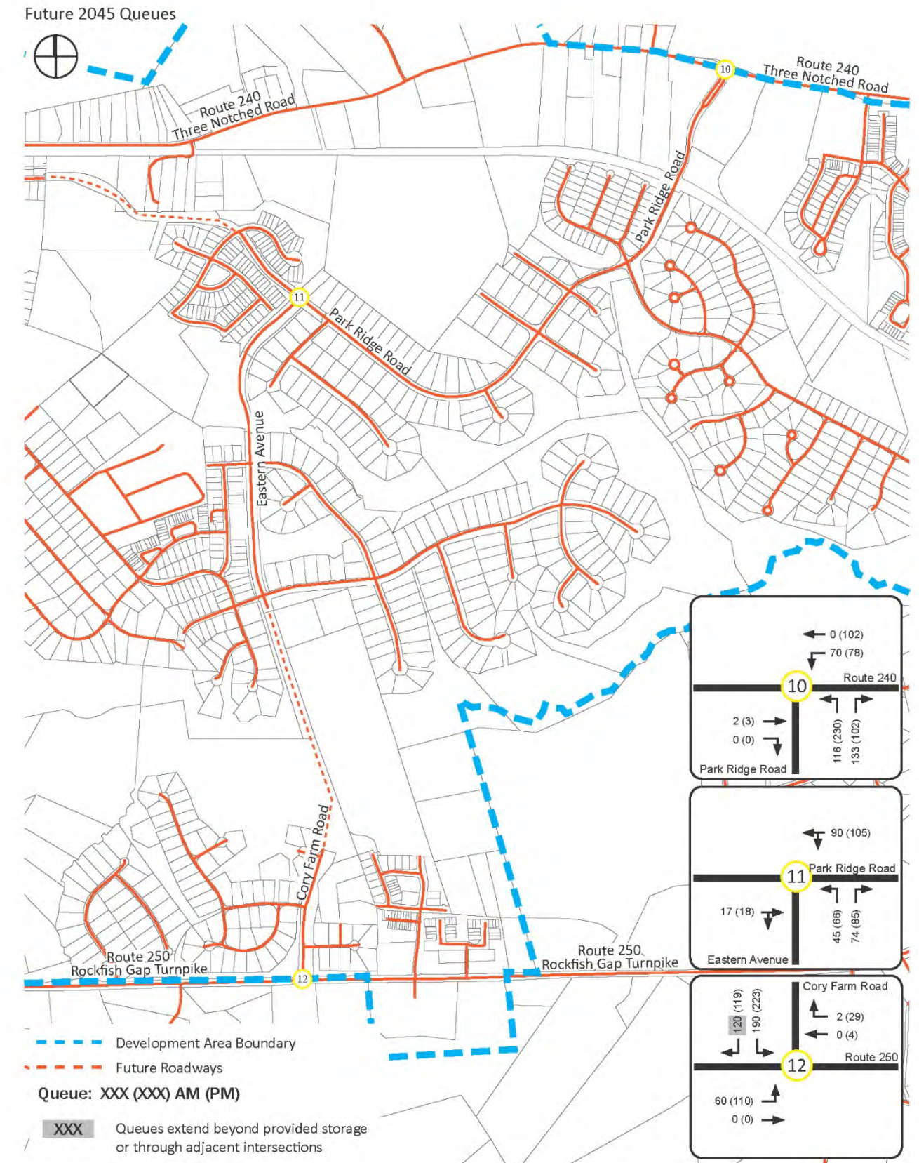
Figure 26 – 2045 Queues Intersections 10-12
